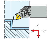
C.-PWLNR/L KAPR = 95,0 °
