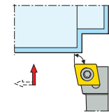
SCFCR/L KAPR = 90,0 °
