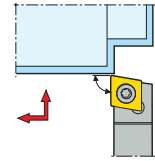
SCACR/L KAPR = 90,0 °
