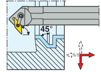
MVYNR/L KAPR = 95,0 °
