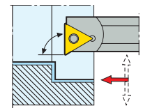
STFDRL/L KAPR = 90,0 °
