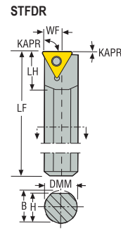
STFDRL/L KAPR = 90,0 °
