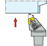
C-DCKNR/L, -M KAPR = 75,0 °
