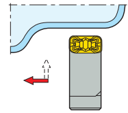
CT-PLFNR/L KAPR = 90,0 °
