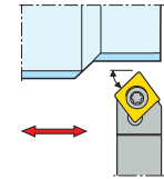
SCFCR/L KAPR = 90,0 °
