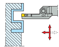
CFOR/L KAPR = 90,0 °
