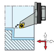
GL..-SCLCR/L KAPR = 95,0 °
