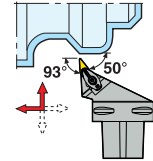
C.-DVJBR/L...JETI KAPR = 93,0 °
