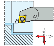
C-SCLCR/L KAPR = 95,0 °
