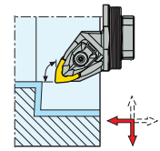
GL..-DWLNR/L KAPR = 95,0 °
