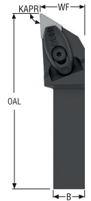
DDJNR/L0.75...JETI
