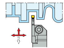
CFIR/L KAPR = 90,0 °
