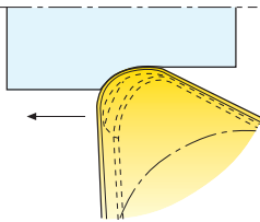
Axial turning (full wiper effect)
